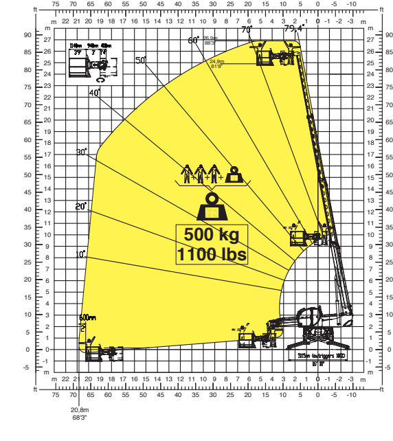
REP 2.2 Vast draai platform 500 kg
